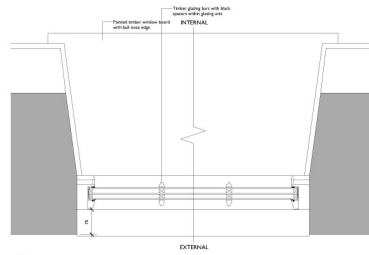
2 BARN 2 Scale: 1:5 OPENING LOWER CASEMENT WITH UPPER FIXED PANES - PLAN
