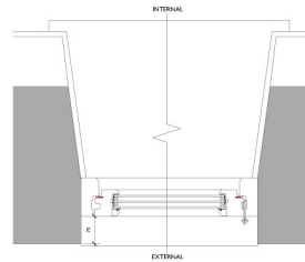
4 OPENING CASEMENT-PLAN Scale: 1:5
