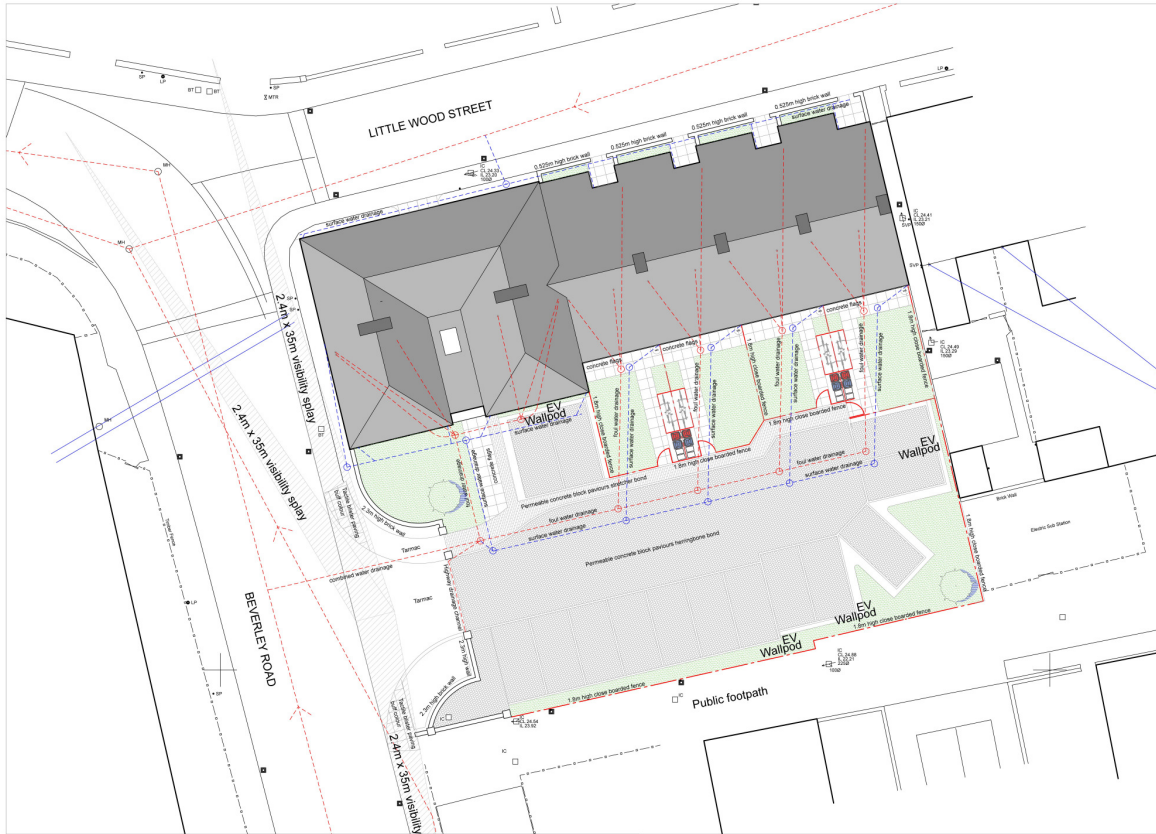
Site Plan Scale 1:100 @ A1
