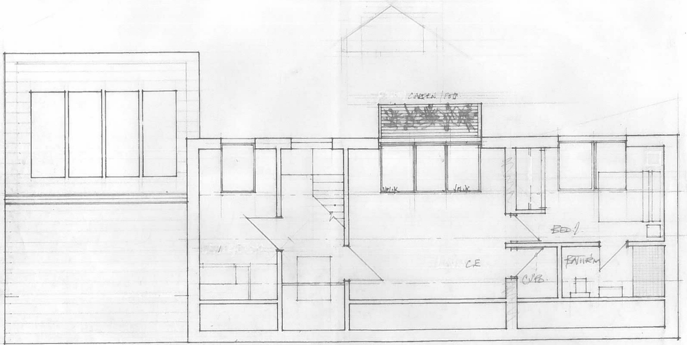
FIRST FLOOR, NEW DWELLING, MARCH COTA LET 88 LEAD EN B C
