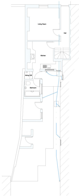
EXISTING GROUND FLOOR PLAN
