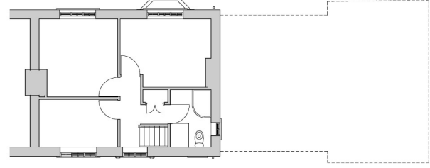
EXISTING FIRST FLOOR 1:50
