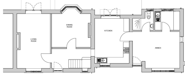
EXISTING GROUND FLOOR 1:50
