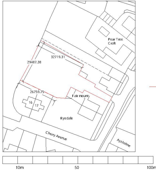
1 Location Plan 1 : 1250
