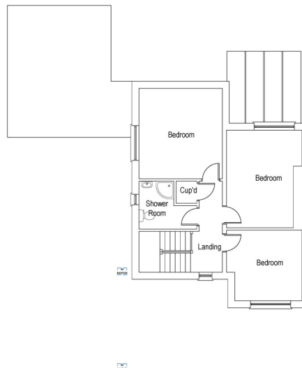
Existing First Floor Plan Scale 1:50
