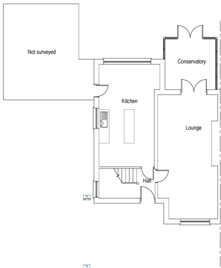
Existing Ground Floor Plan Scale 1:50
