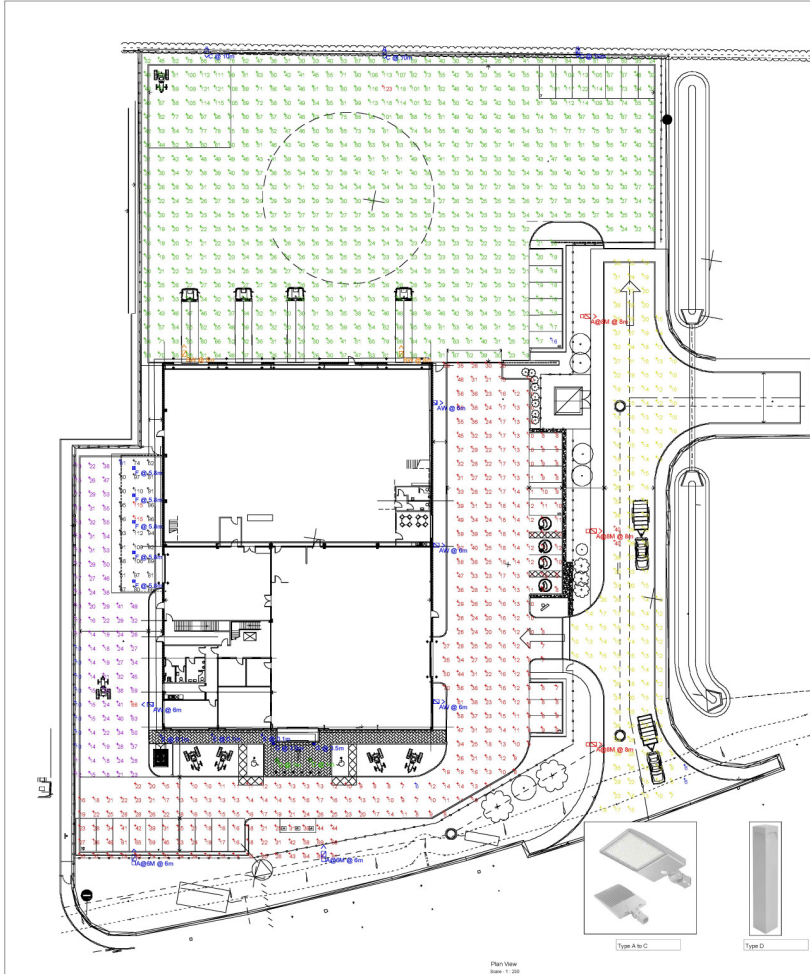
Plan View Scale: 1:250
