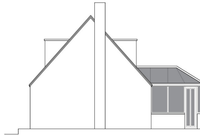
2 Existing Side Elevation 04 1:50
