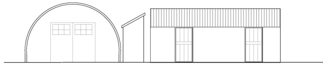
1 Front Elevation 12 1:50
