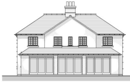
South Elevation
