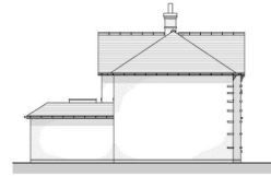
East Elevation
