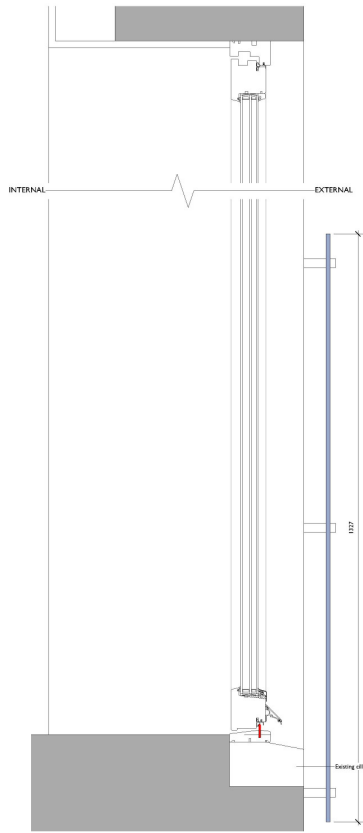
1 BARN_2 Scale: 1:5 CASEMENT WINDOW WITH GLASS BALUSTRADE - SECTION
