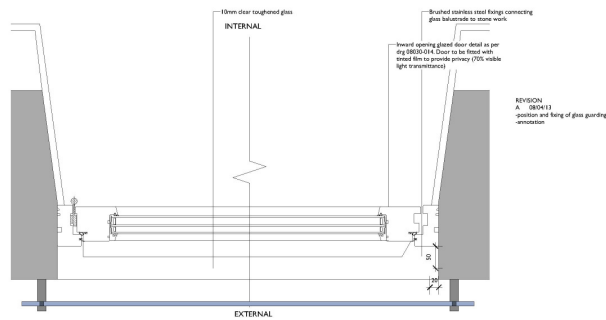
3 BARN_2 Scale: 1:5 CASEMENT WINDOW WITH GLASS BALUSTRADE - PLAN
