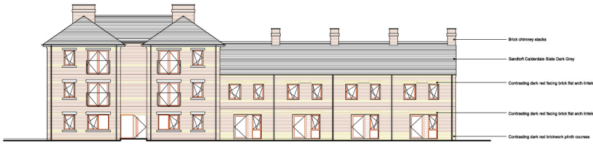
SOUTH ELEVATION
