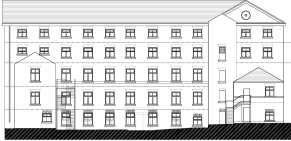
EAST ELEVATION (COURTYARD)
