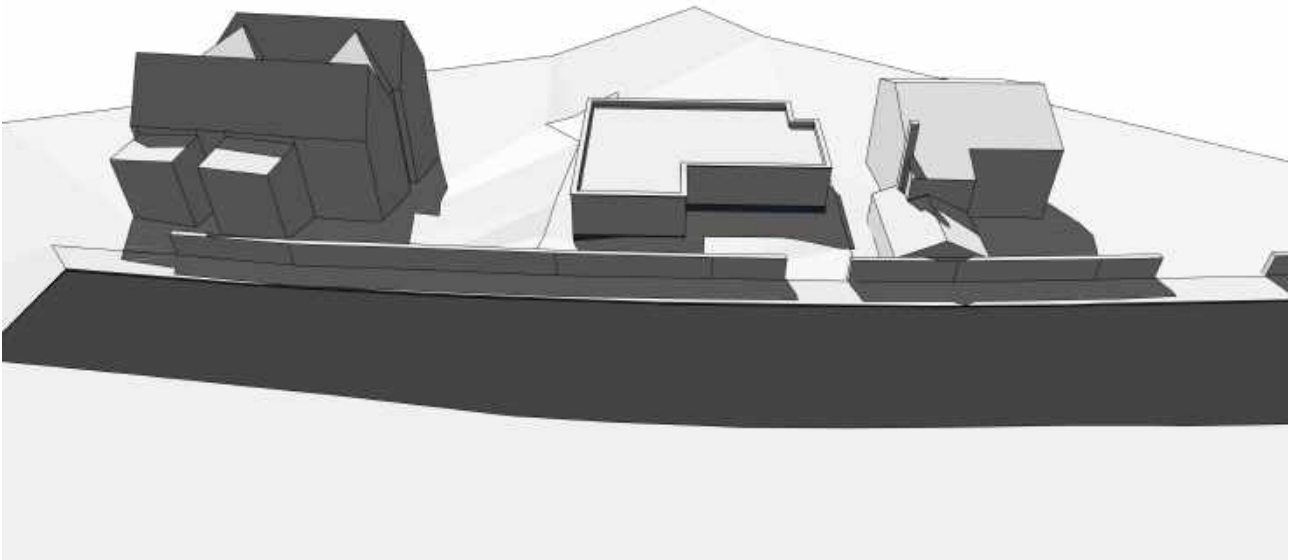
Existing 09:00 June 21st
