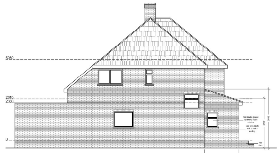
Proposed Southwest Elevation Scale 1:50
