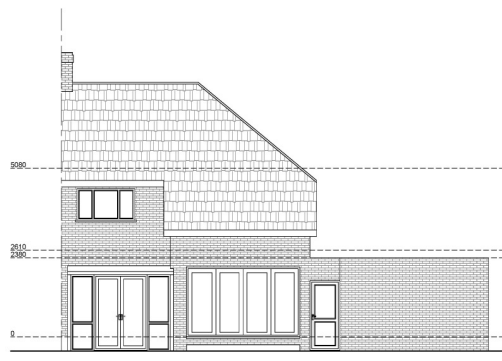
Proposed Northwest Elevation Scale 1:50
