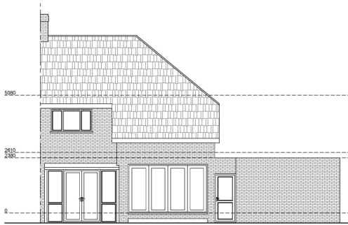
Existing Northwest Elevation Scale 1:50
