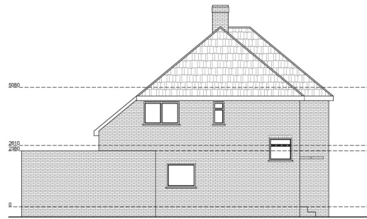
Existing Southwest Elevation Scale 1:50
