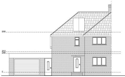
Existing Southeast Elevation Scale 1:50
