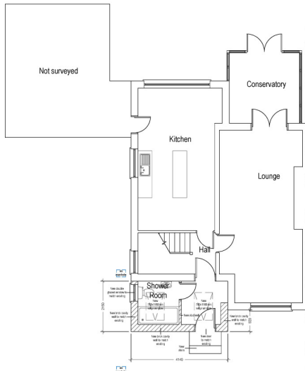
Proposed Ground Floor Plan Scale 1:50
