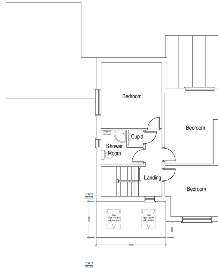
Proposed First Floor Plan Scale 1:50
