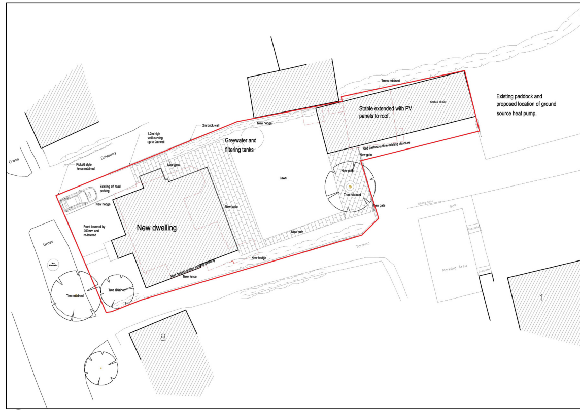
1 Site Layout Existing and Proposed 03 1:100
